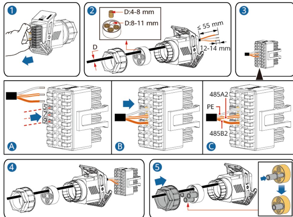
Figure 5-29 Installation du câble
